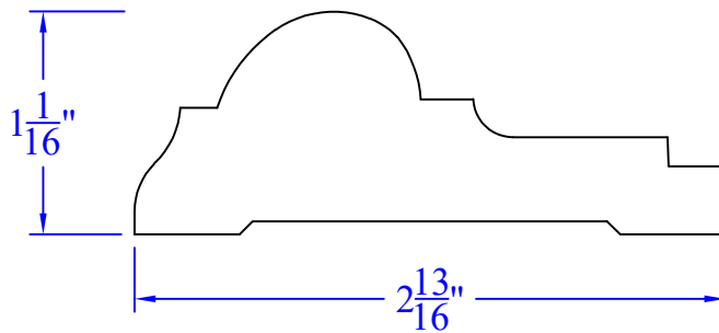
CASG1006 1\frac{1}{16} " x 2\frac{13}{16} "
