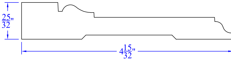
CASG330 \frac{25}{32} " x 4\frac{15}{32} "
