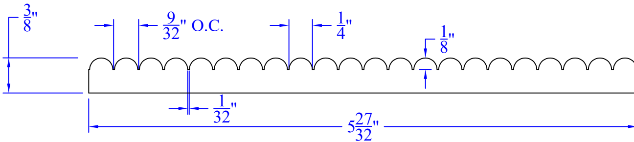
MLDG112 \frac{3}{8} " x 5\frac{27}{32} "
