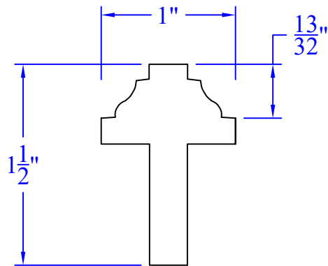
WTRM075 1-1/2" x 1"
